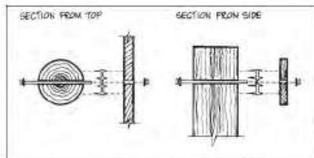
Figure 4.34. Spiked Grid
