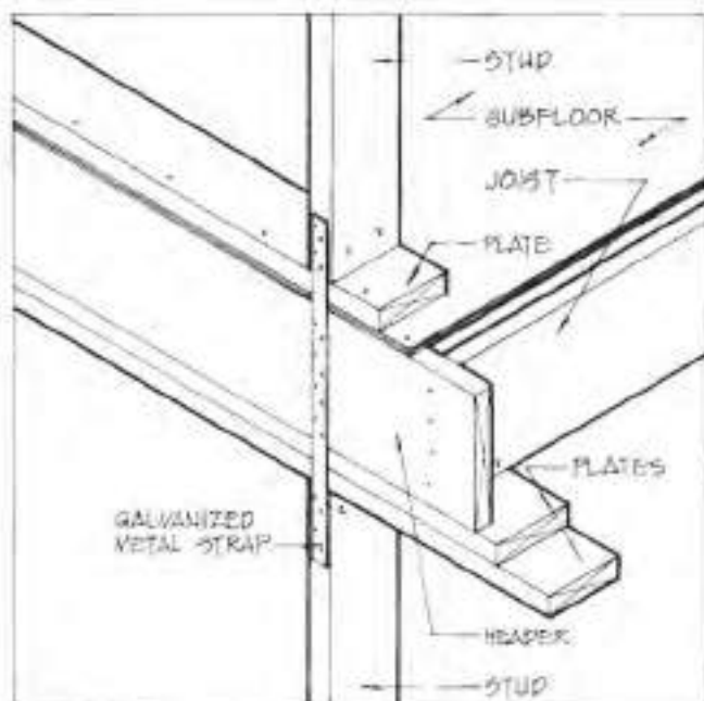
Figure 4.44. Stud-to-Stud Connections
