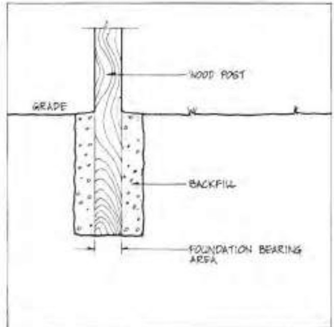
Figure 4.6. Earth Bearing
