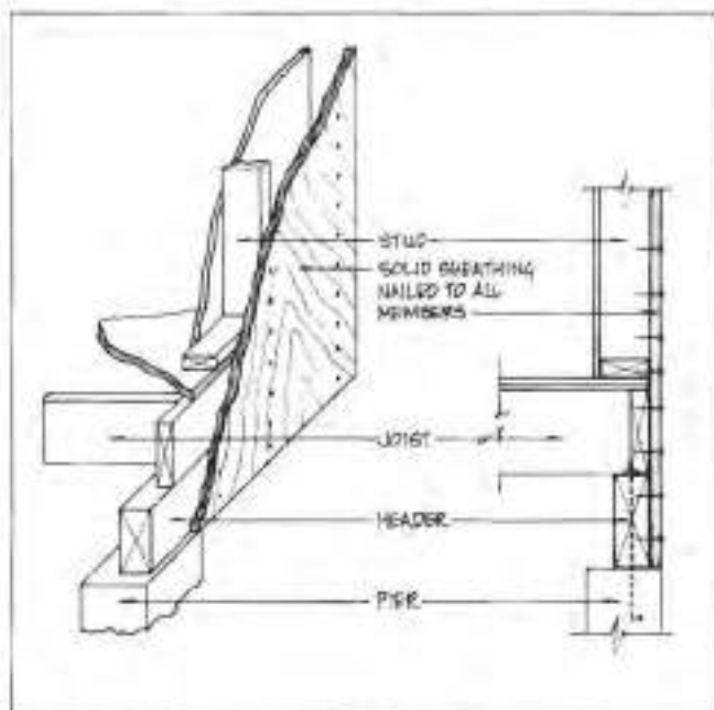
Figure 4.45. Plywood Anchorage
