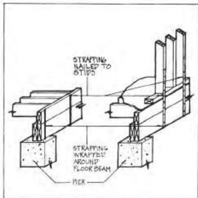
Figure 4.43. Metal Strapping
