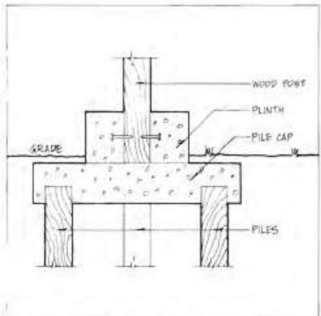
Figure 4.8. Post/Pile Foundation
