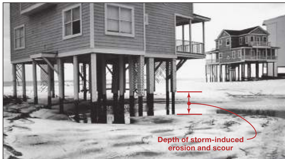
Figure 3-21. Pile-supported house in the area of channeled flow shown in Figure 3-20. The building foundation and elevation successfully prevented high-velocity flow, erosion, and scour from destroying this building
